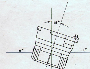
CONDITION AFTER ATTACKS FRAME 112 → LOOKING FORWARD DRAFT UNDETERMINED HEEL AT 1650 → 18°
