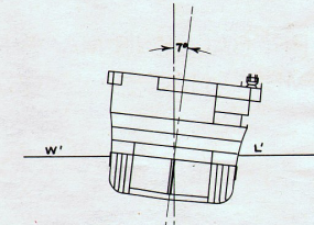
CONDITION BEFORE ATTACKS FRAME 112 → LOOKING FORWARD MEAN DRAFT-30.5' HEEL-7°
