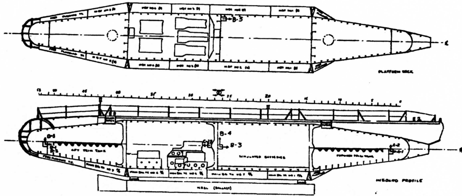
Fig. 3.64—Plan view and inboard profile of SQUAW, showing general layout, instrument locations, and orientations.
