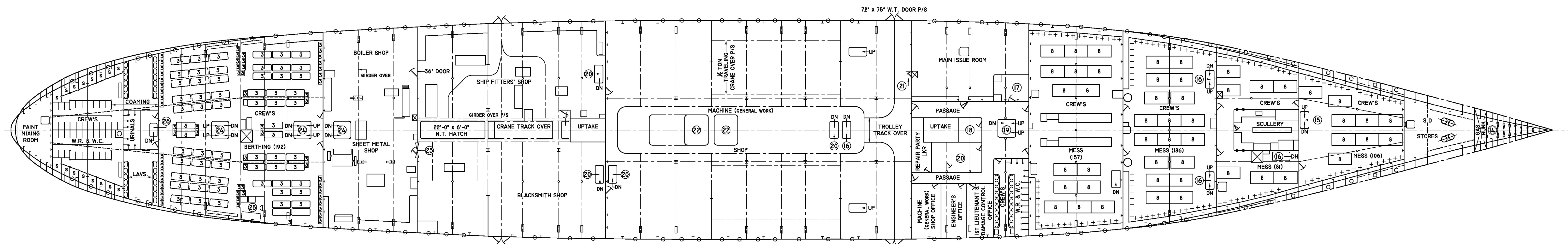
SECOND DECK
