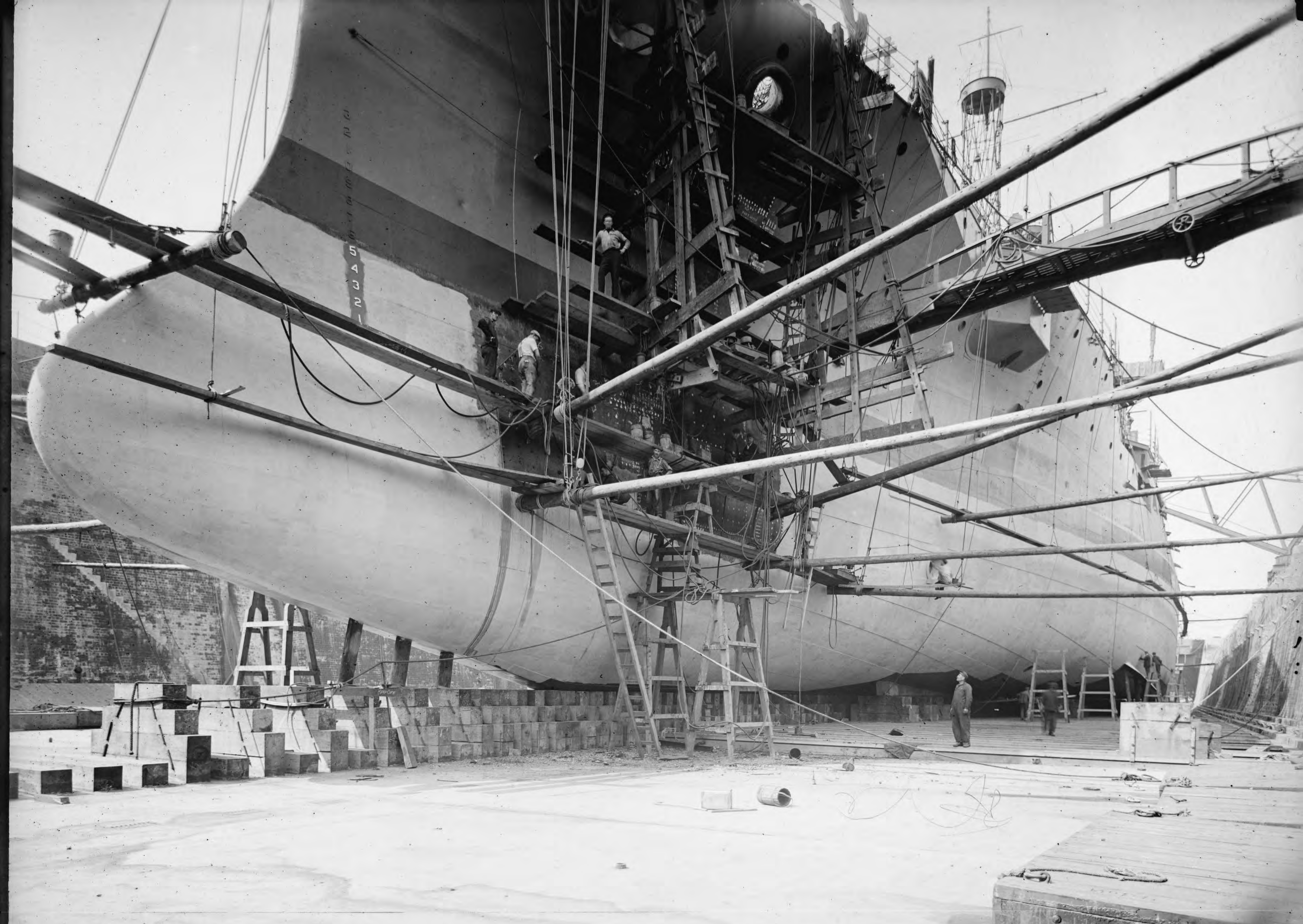
F544 N785, NAVY YARD, NEW YORK, 5-24-12, U. S. S. UTAH-FIRST DOCKING IN DRY DOCK NO. 4,
