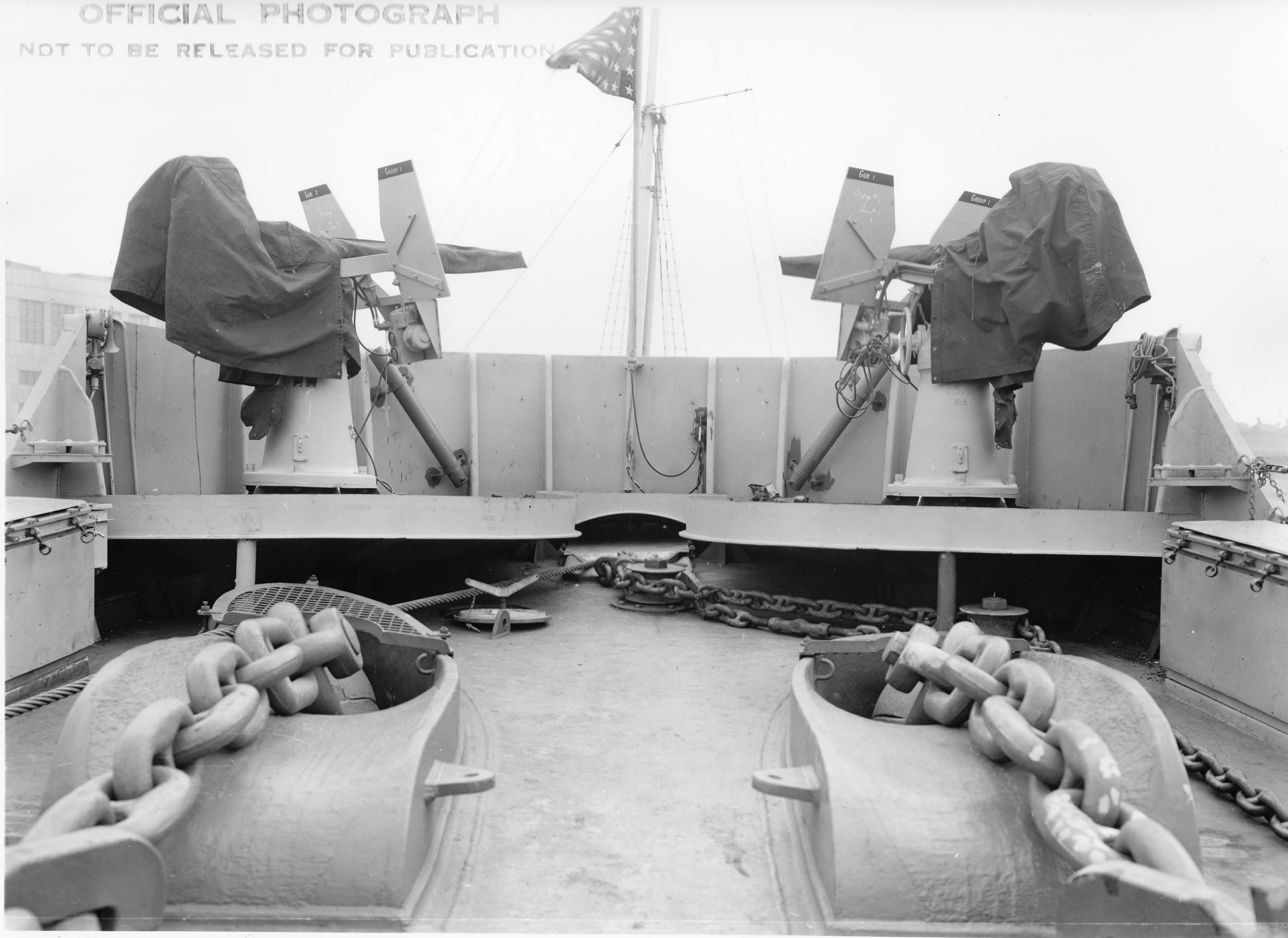
F1111C474 U. S. S. BB 61. 20 MM. MOUNTS AT BOW. MAIN DECK LOOKING FORWARD.
