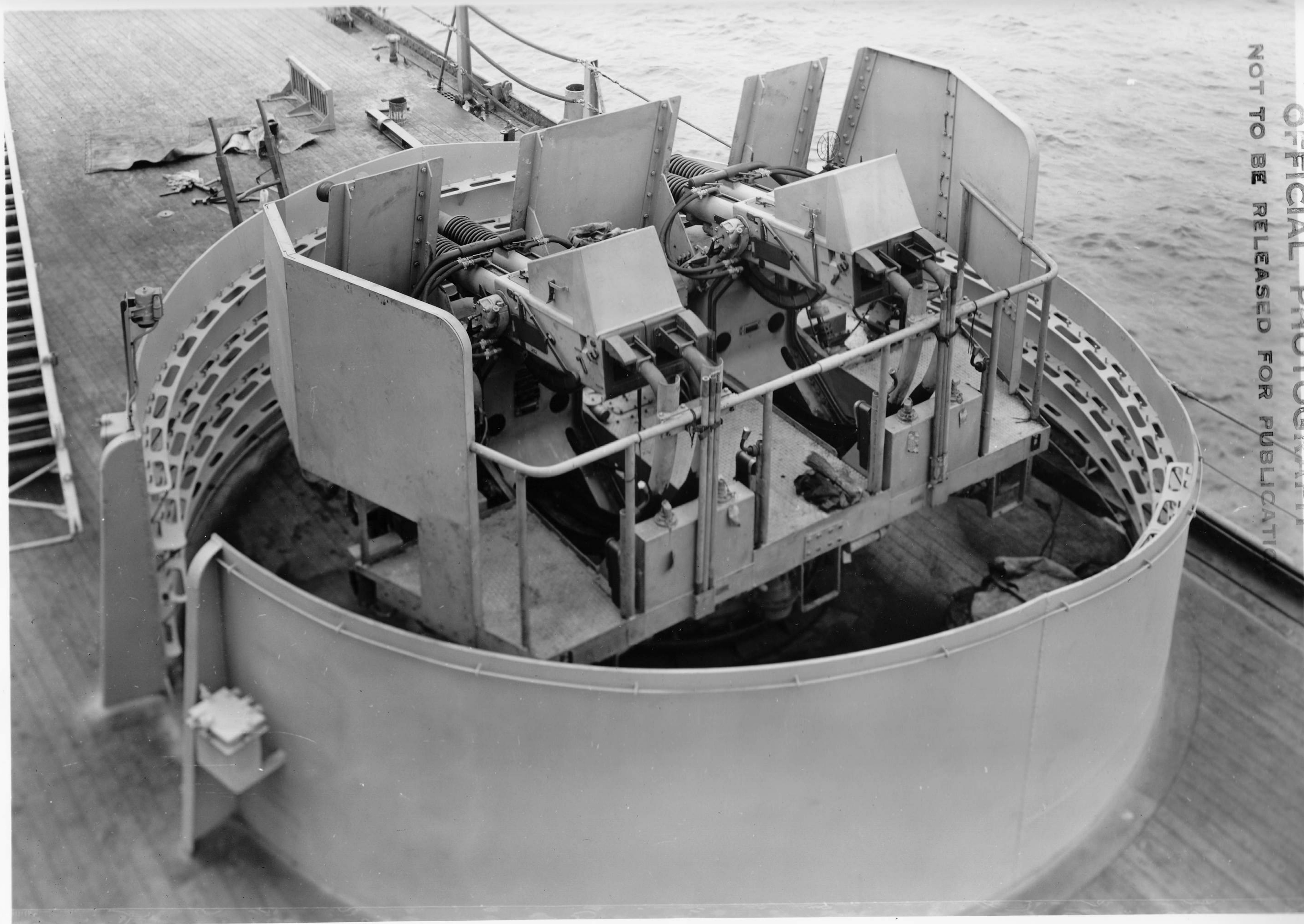
F1111C472 U. S. S. BB 61. 40 MM. MT. MAIN DECK FR. #145 (P). TOP VIEW LOOKING AFT.
