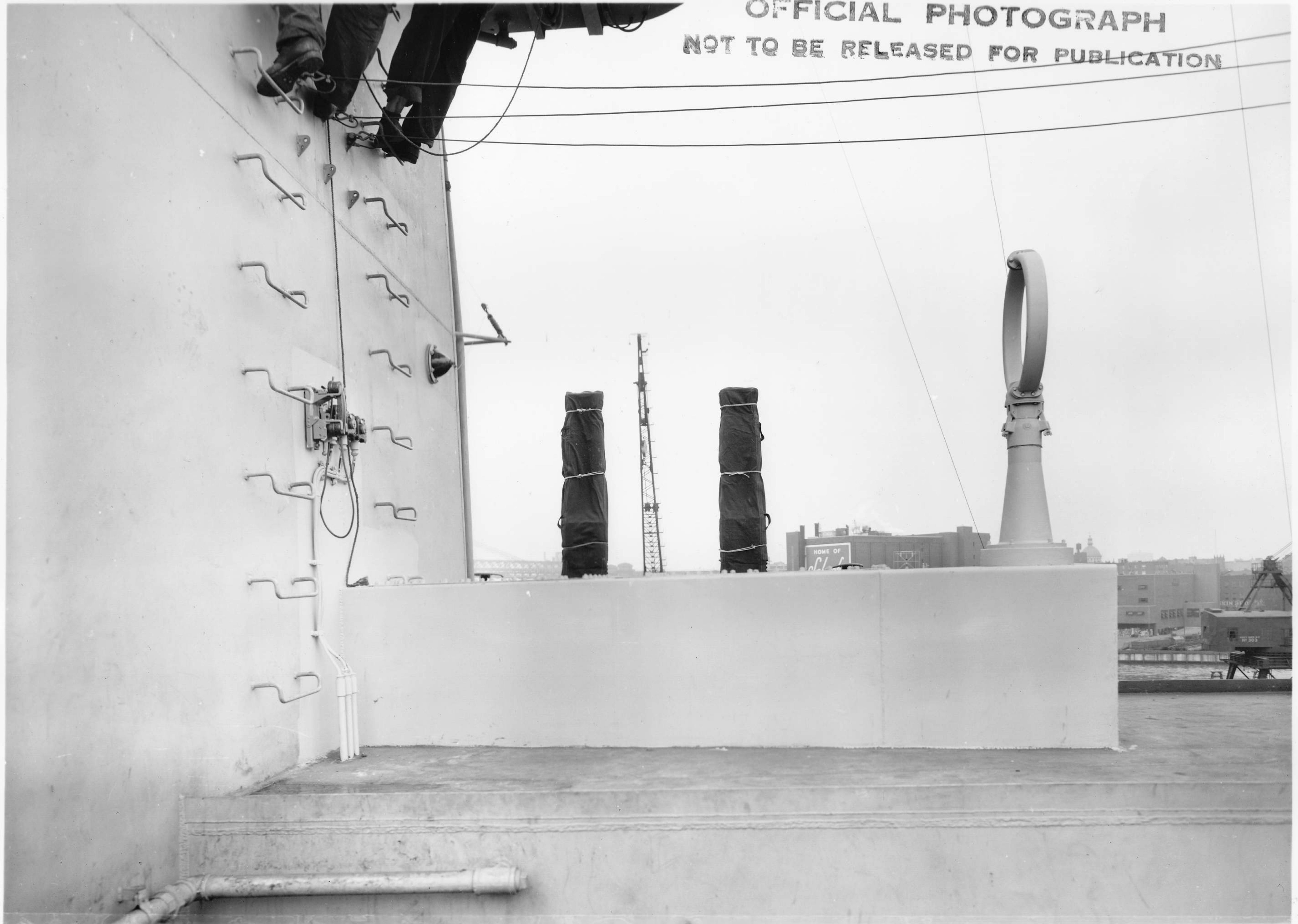
F1111C461 NAVY YARD, NEW YORK JULY 9, 1943 U. S. S. BB 61 R. D. F. LOOP & TRUNK. 1st LEVEL ABOVE P. H. TOP FR. 97, LOOKING TO PORT.
