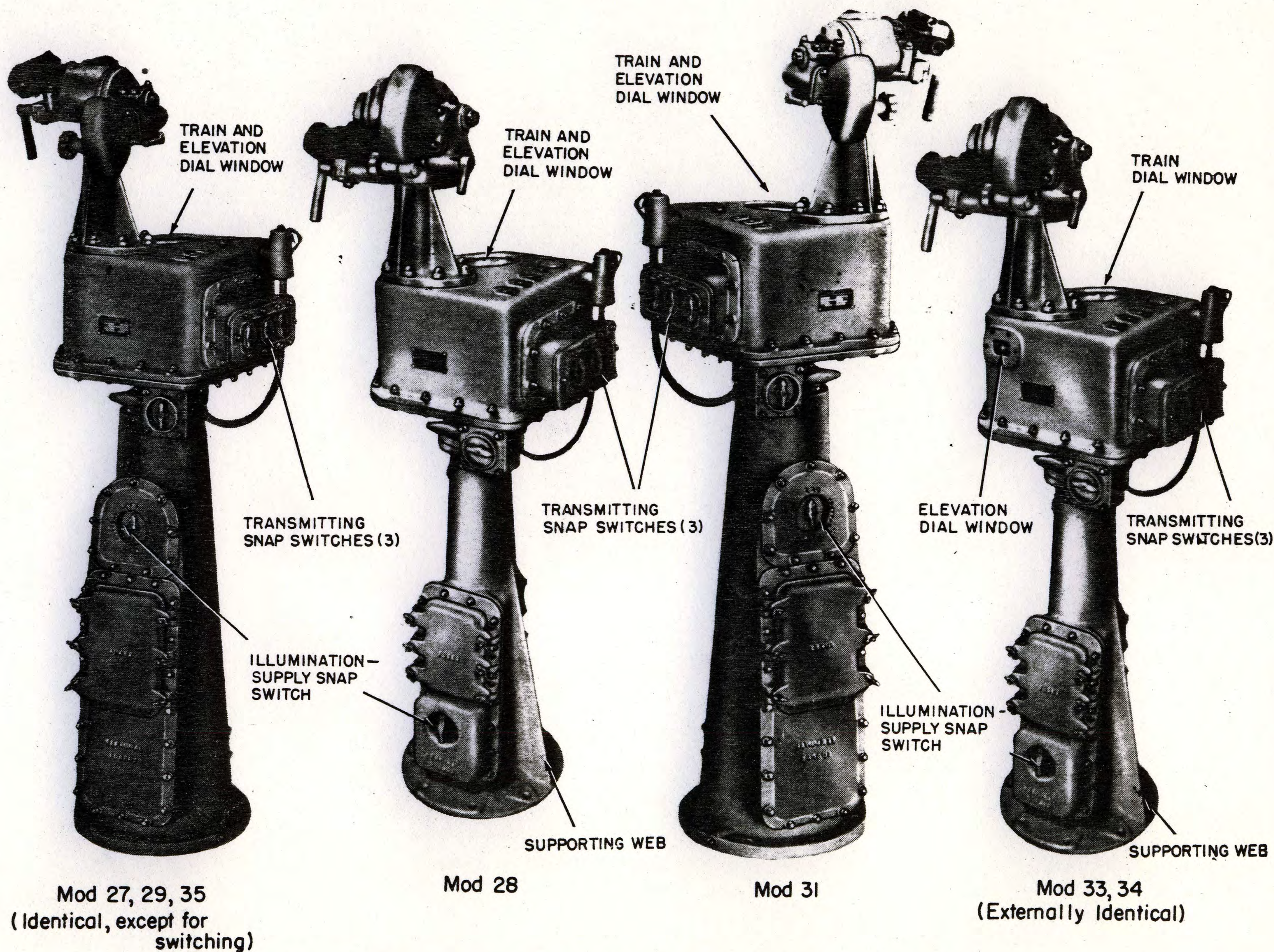
Figure 6.—Target Designation Transmitter and Receiver Mk 1 and Mods. External Appearances.
