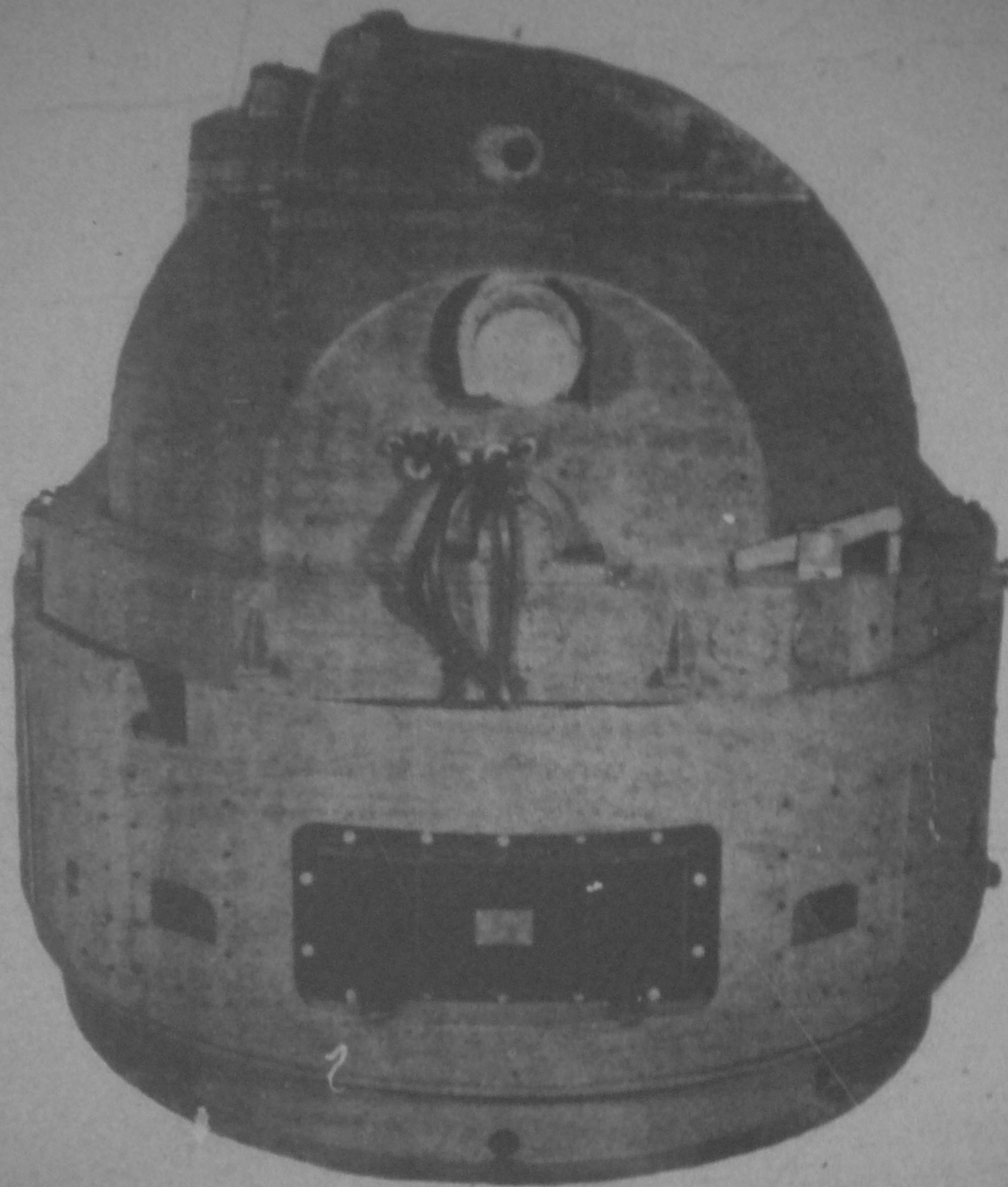
GUN DIRECTOR MARK 45 Left Side View - 0° Elevation
