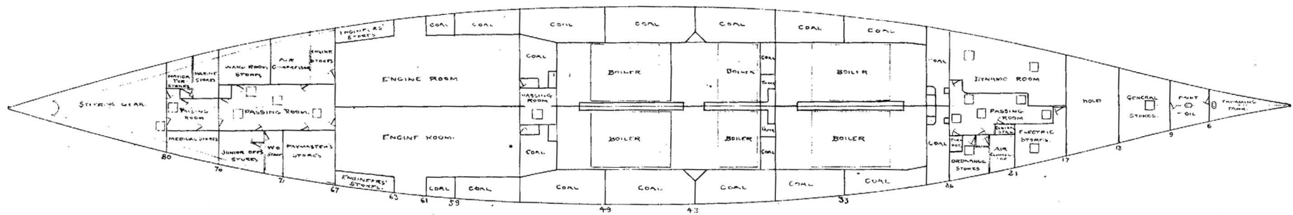
— PLATFORM DECK — SCALE \frac{1}{24} " = ONE FOOT
