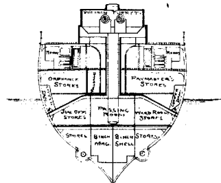
— SECTION AT — — FRAME NO 73 —
