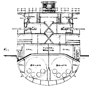
— SECTION AT — — FRAME NO 30 —
