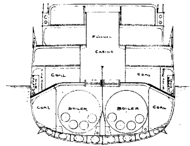
— MIDSHIP SECTION — SCALE \frac{1}{24} " = ONE FOOT
