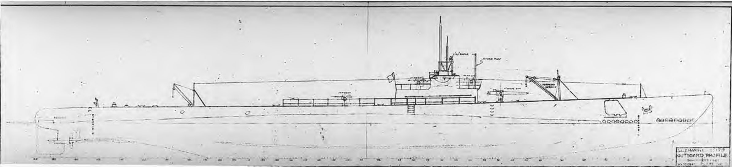
Photo # NH 79457-A USS Plunger (SS-179) Booklet of General Plans, 8 December 1943. Sheet 3: Outboard Profile
