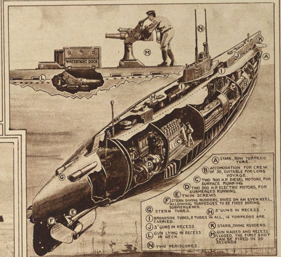
CROSS SECTION OF A GERMAN SUBMARINE SHOWING EVERY IMPORTANT FEATURE THAT HAS MADE IT SUCH A MENACE DURING THE WAR.
