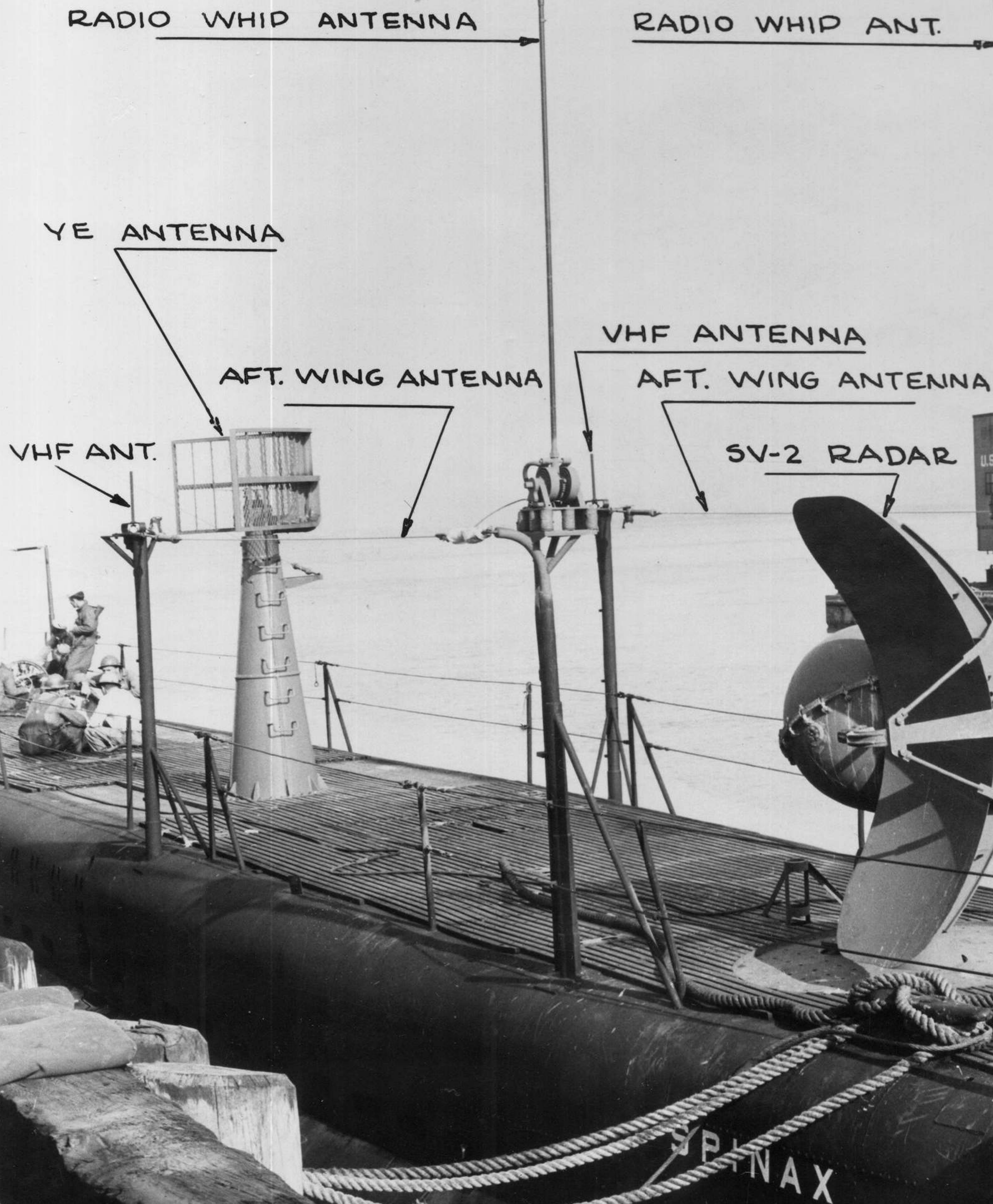
NY1-306-(G-S)-11-14-50 SSR489 (SPINAX) AFT ANTENNA ARRANGEMENT LOOKING FORWARD FR. PORT STERN SAN FRANCISCO NAVAL SHIPYARD
